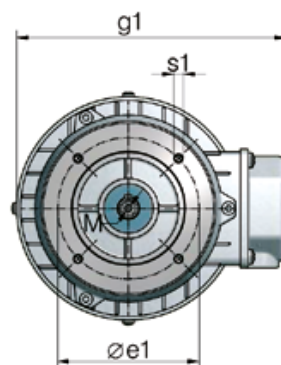
B14: Flange with internal thread C: Small flange
