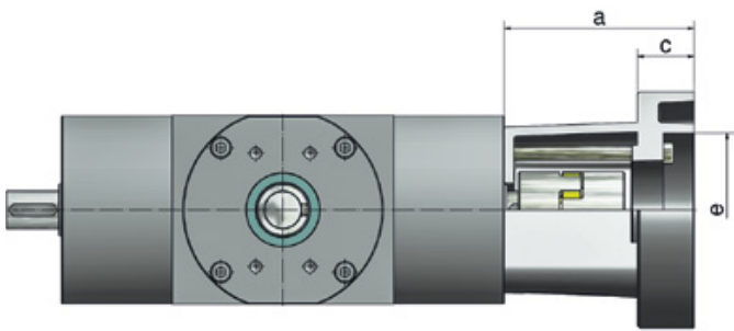
Motor flange base MF-B and motor flange plate MF-P - KSZH-50 to KSZ-H-150 (2 pieces)
