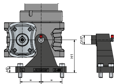
Pivot mount LB (50 - 200 kN)
