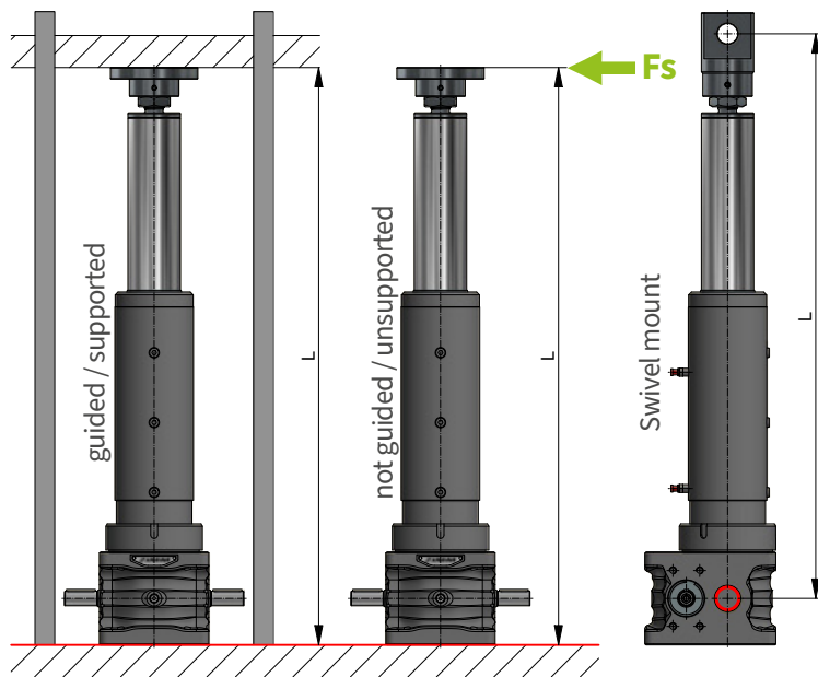
Critical buckling force ZA-100
