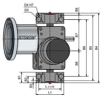
Pivot mount LB (25 kN)
