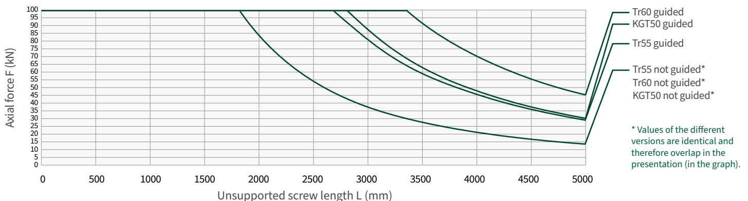
Critical buckling force ZA-100
