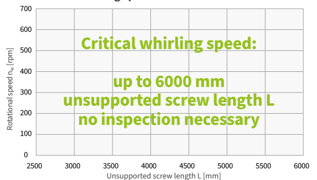
Critical whirling speed ZA-100
